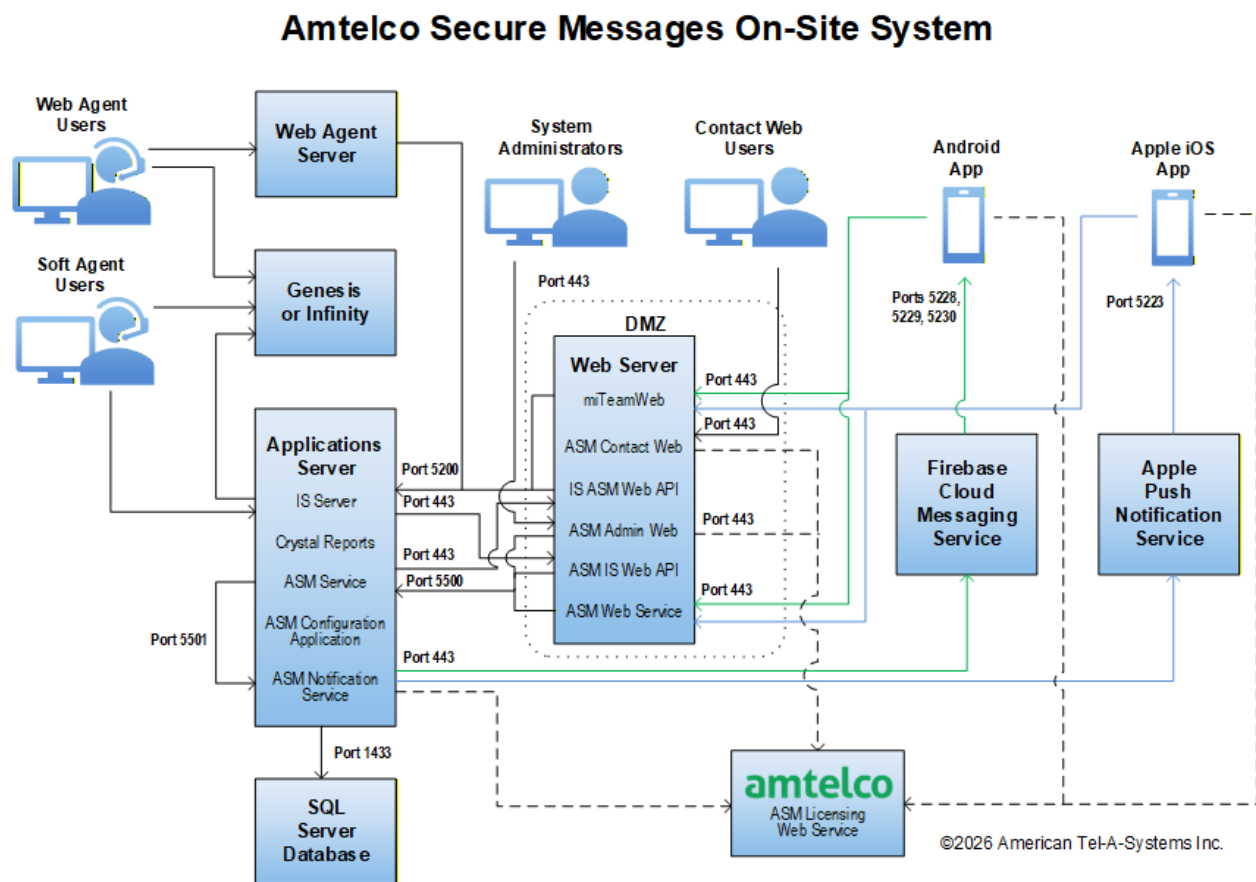
Amtelco Secure Messages in a complete on-site environment with IS 5.7
