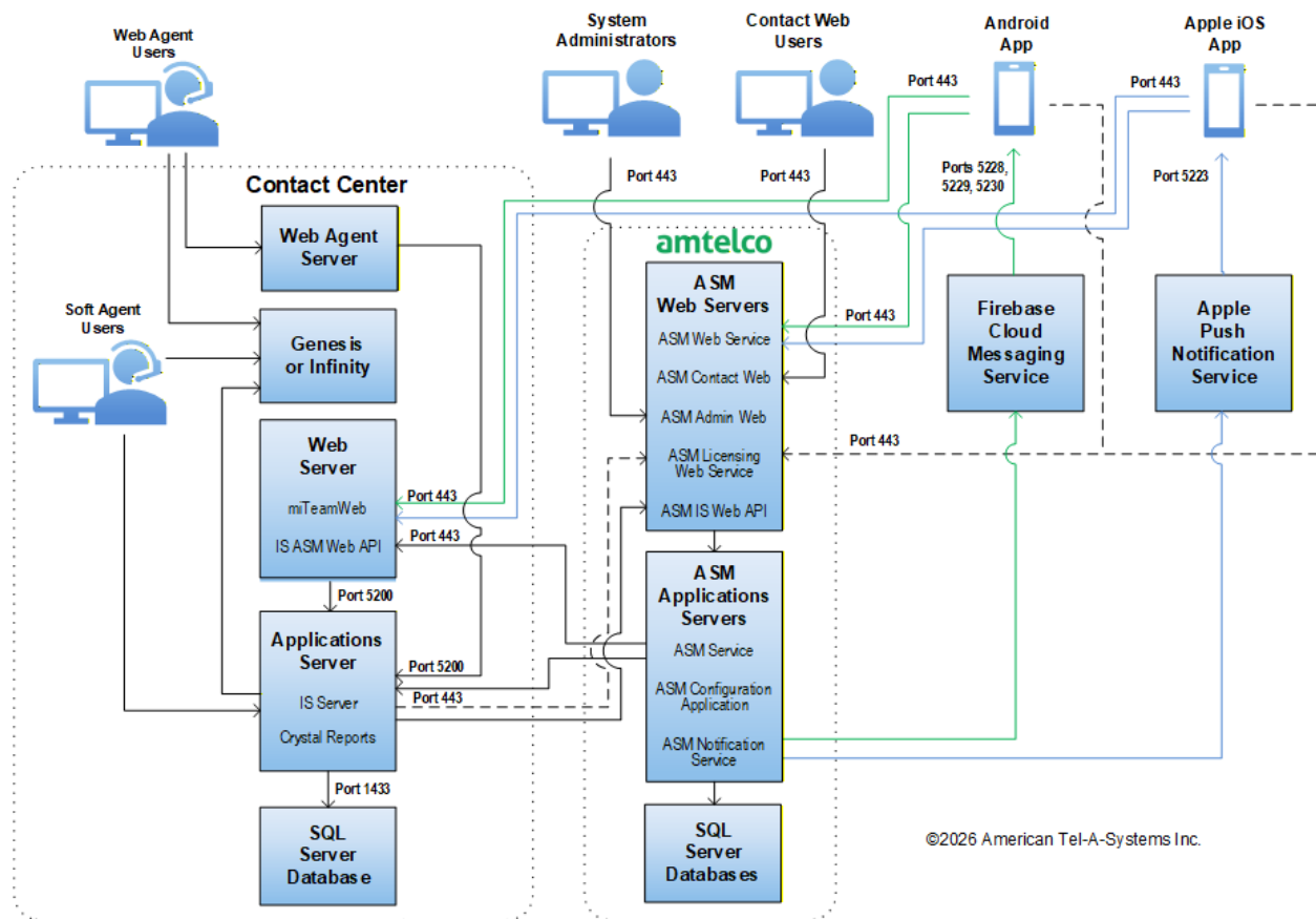
Amtelco Secure Messages cloud-based solution with on-site IS 5.7
